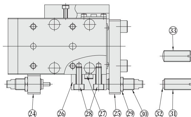
MGA□10~□20 (with shock absorber)
