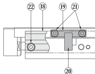
MGA□10~□20 (with shock absorber)
